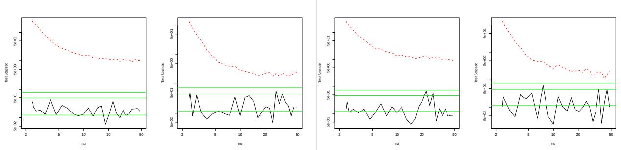
Figure 3: Cramér-von-Mises statistics test of N(0,1) for \hat{T}_{\hat{\beta}} (black line) and \hat{T}_{LS} (dotted red line) for various values of n , \nu and \sigma . Throughout 500,000 replications are used. Green horizontal lines represent the 0.5, 0.95 and 0.99 quantiles of the Cramer-Von-Mises statistic when the data is i.i.d. N(0,1) . Results to the left hand side have \sigma = 2 , and results to the right have \sigma = 4 . 1st and 3rd graph have n = 100 ; 2nd and 4th have n = 250 . Throughout the x -axis is \nu , on the log-scale. The y -axis is also drawn on the log-scale.
