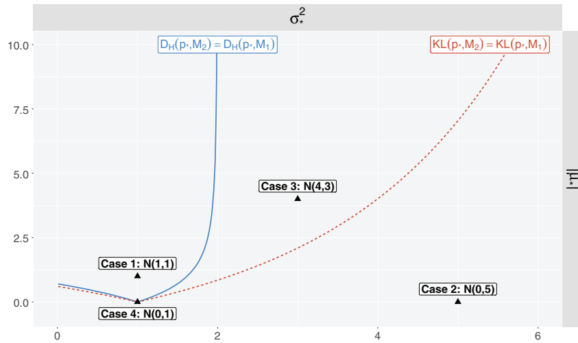
Figure 2. Phase plane of d(p_*, M_2) - d(p_*, M_1) as a function of (|\mu_*|, \sigma_*^2) , where d \in \{D_H, KL\} . The four cases from Section 2.3 are indicated as triangles. The lines (solid for D_H , dashed for KL ) are the sets of (|\mu_*|, \sigma_*^2) such that d(p_*, M_2) = d(p_*, M_1) . The regions above (resp. below) the lines satisfy d(p_*, M_2) > d(p_*, M_1) (resp. < ), that is, M_1 (resp. M_2 ) is closer to p_* .
