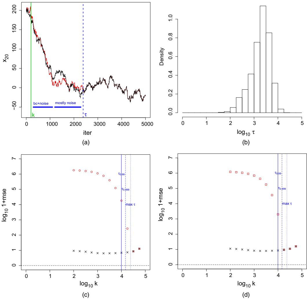
Fig. 9. Plots from the experiment described in the text: (a) first 5000 iterations of the first simulation ( \tau ; k , putative k ); (b) histogram of all 5000 values of \log_{10}(\tau) ; (c) \log_{10}(1 + \text{MSE}) (mean taken over the 5000 simulations) of unbiased MCMC ( \circ ) and MCMC ( \times ) sampling as a function of k ( \tau_{0.99} ; \tau_{0.999} ; \max \tau (not \tau_{\max} ) value over the 5000 simulations); (d) \log_{10}(1 + \text{MSE}) of Rao-Blackwellized unbiased MCMC ( \square ) and MCMC ( \times ) as a function of k
